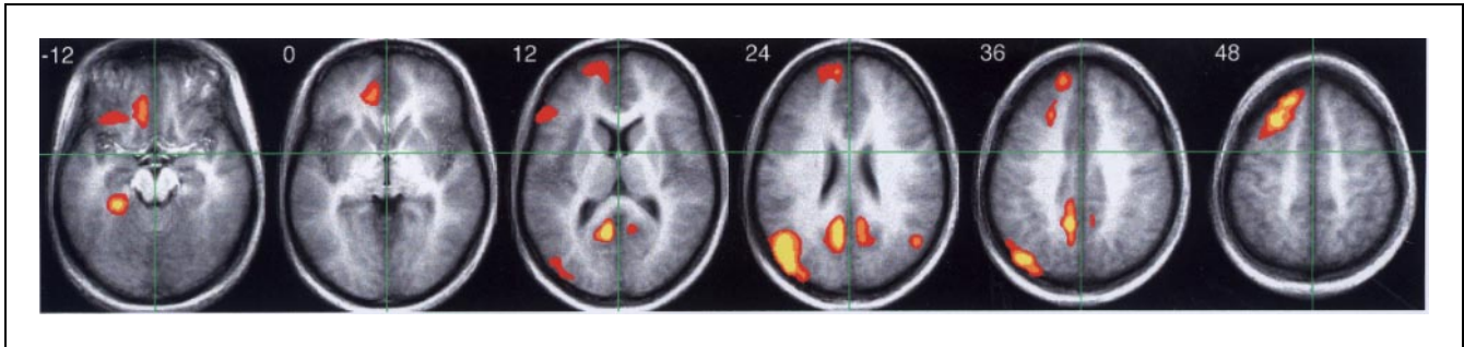
Figure 1. Rest minus Tones. Regions of significant activation difference ( p < 0.00001 ) are shown in red-yellow superimposed on averaged anatomical brain images in axial orientation. Stereotaxic x and y axes are shown in green, and z coordinates are given above each image. The left hemisphere is on the reader's left. Areas more active during rest include the left parahippocampus ( z = -12, 0 ), orbital frontal and rostral-ventral anterior cingulate cortex ( z = -12, 0 ), left > right angular gyrus ( z = 12, 24, 36 ), left > right posterior cingulate/retrosplenial cortex ( z = 12, 24, 36 ), and left dorsal prefrontal cortex ( z = 12, 24, 36, 48 ).
